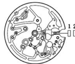
TY2809 (1601K3) 21 Jewels
